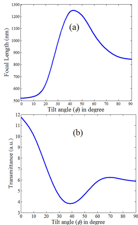
FIG. 6 (a) The focal length versus tilt angle (b) The transmittance versus tilt angle
