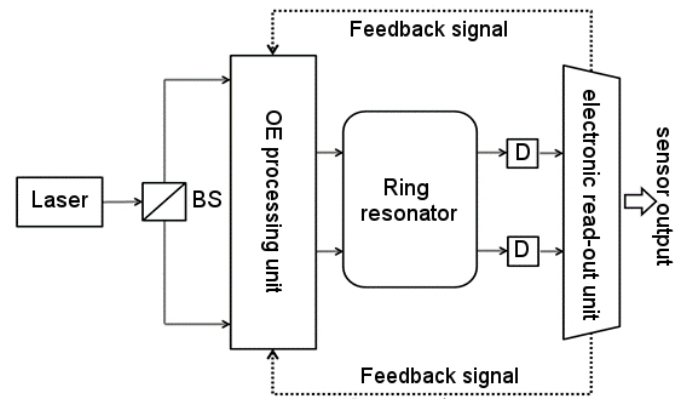
FIG. 7 Configuration of a Resonant Micro-Optic Gyroscope (RMOG), including a laser, a Beam Splitter (BS), Opto-Electronic (OE) components for signal processing, a ring resonator, two detectors (D) and an electronic read-out unit.
