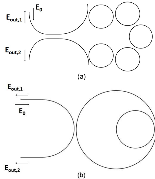
FIG. 15 Different configuration of multi ring structures proposed as sensing element of gyro: (a) CROW structure with five identical ring resonators, and (b) folded structure with two nested ring resonator having one the half radius of the other.
