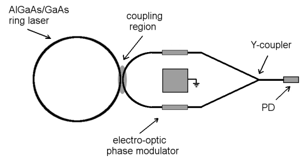
FIG. 4 Configuration of the SRL based gyro chip (3 mm x 5 mm) on GaAs [37].
