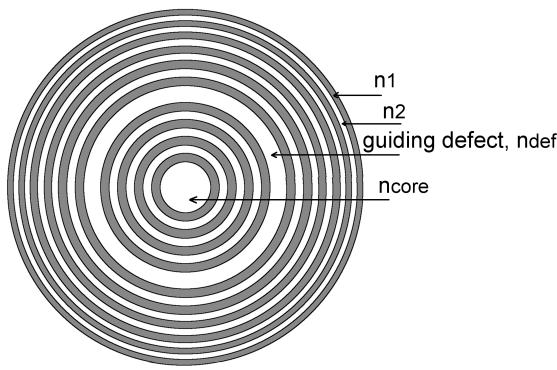
FIG. 6 Circular Bragg laser with a circular guiding defect, having refractive index n_{def} , surrounded by two Bragg reflectors in which dark rings have refractive index n_1 and white rings n_2 < n_1 [39].
