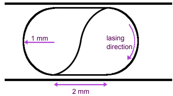
FIG. 2 Racetrack Semiconductor Ring Laser (SRL) with S section.
