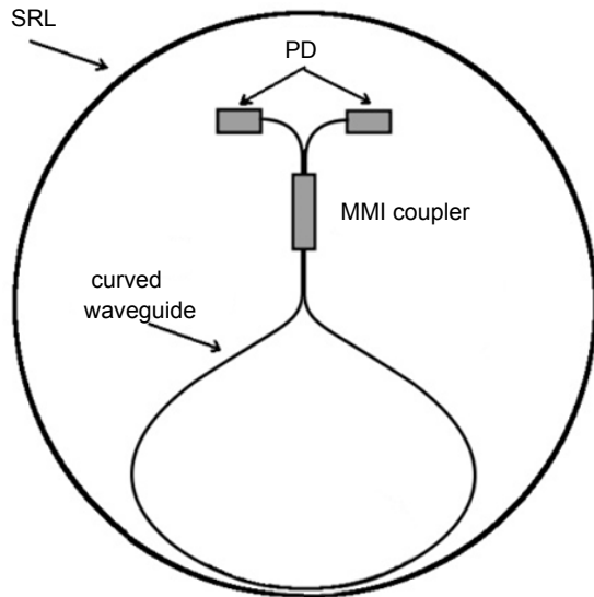
FIG. 3 Compact configuration of an SRL based gyro [29, 30] that includes an SRL inside of which there are a curved waveguide, an MMI coupler and two photodetectors for the system read-out.
