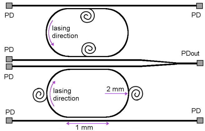
FIG. 5 Active gyroscope realized with two unidirectional racetrack SRL inside of which spiral waveguide sections prevent lasing in the undesired direction.
